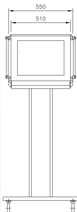
PEDESTAL
