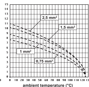
CX 12 D inserts max. current load derating diagram, stamped contacts
