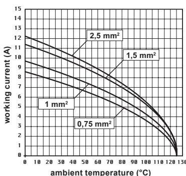
CX 12 D inserts max. current load derating diagram, turned contacts
