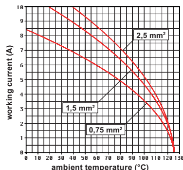
CT 40 inserts max. current load derating diagram
