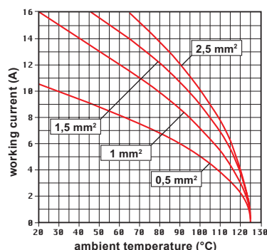
CT 10 inserts max. current load derating diagram
