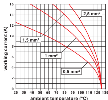
CT 06 inserts max. current load derating diagram
