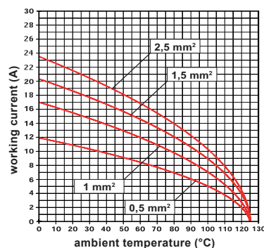
CSH 10 inserts max. current load derating diagram
