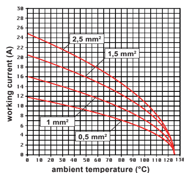
CSAH 10 inserts max. current load derating diagram
