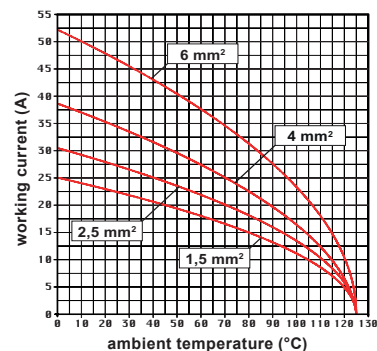
CP 06 inserts max. current load derating diagram
