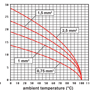
CK 04 inserts max. current load derating diagram
