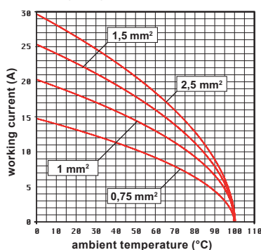
CK 03 inserts max. current load derating diagram
