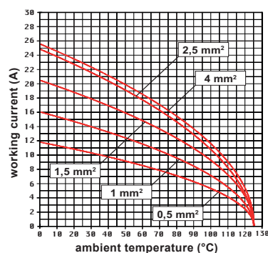
CDA 10 inserts max. current load derating diagram
