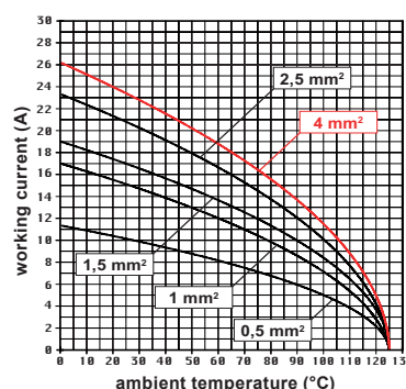
CCE 10 inserts max. current load derating diagram
