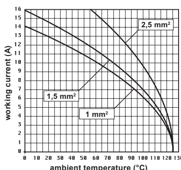
CD 08 inserts max. current load derating diagram, turned contacts
