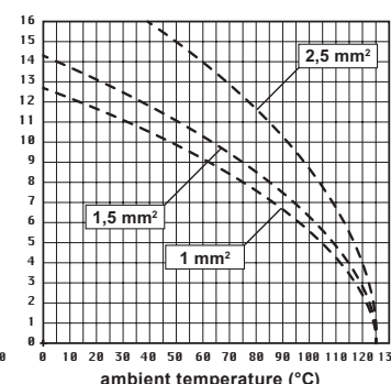
CD 08 inserts max. current load derating diagram, stamped contacts
