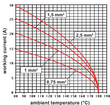
CK RY 03 inserts max. current load derating diagram
