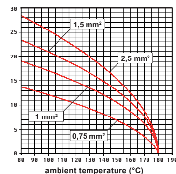
CK RY 04 inserts max. current load derating diagram
