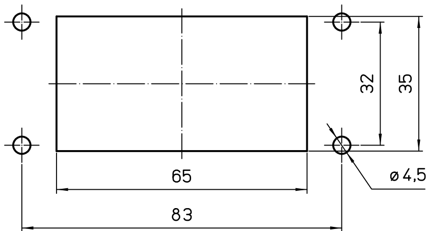
Panel cut-out
