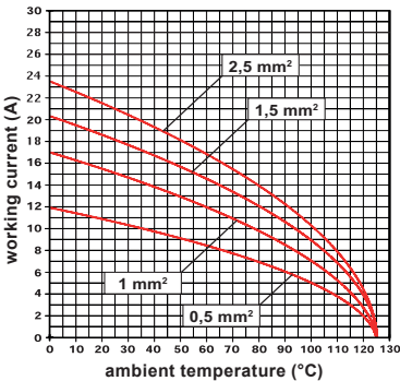
RSH 10 inserts max. current load derating diagram
