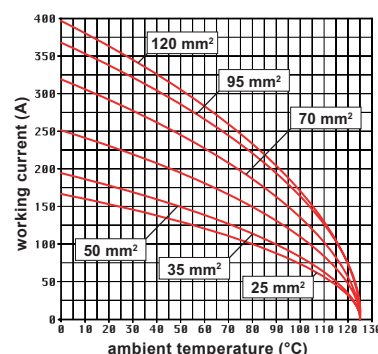
CX 01/01B 30 inserts max. current load derating diagram
