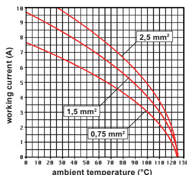
CT 64 inserts max. current load derating diagram
