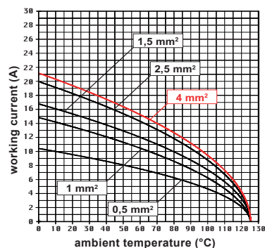
CNE 16 T inserts max. current load derating diagram
