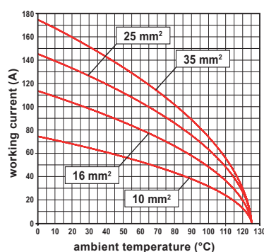
CX 01 G inserts max. current load derating diagram)
